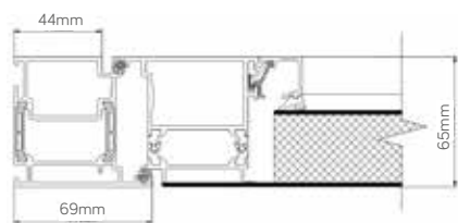
SIDE JAM OPENING IN
