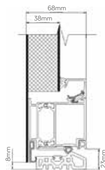
FOOT DETAIL OPENING OUT
