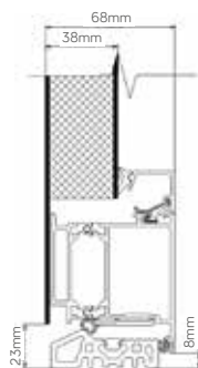
FOOT DETAIL OPENING IN
